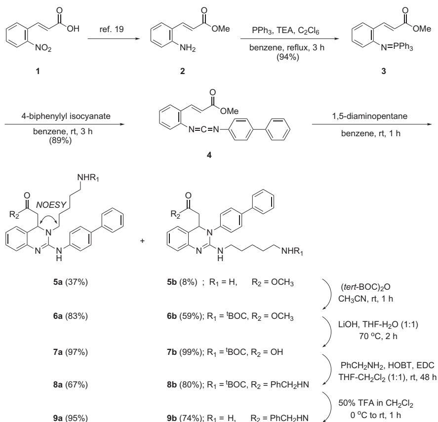
Scheme 1. Synthesis of 3,4-dihydroquinazoline derivatives.
