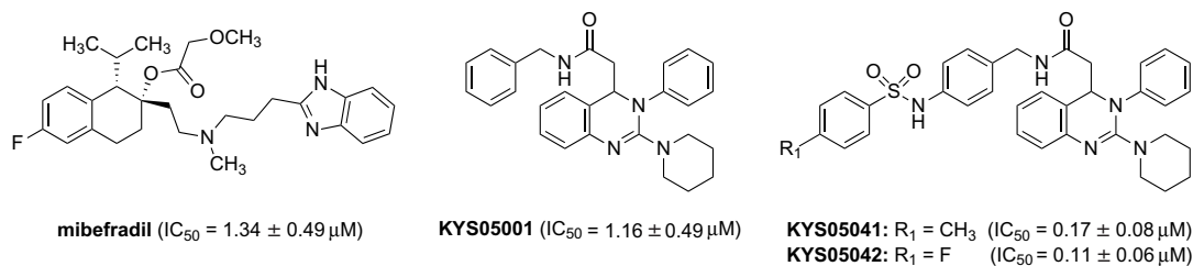
Figure 1. Structures of some T-type Ca^{2+} channel blockers.
